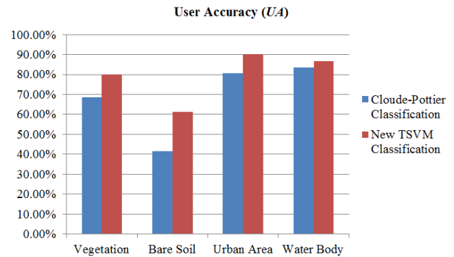
Fig. 5. UA of two classification methods over four land covers
