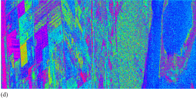
Fig. 3. The decomposition results of Cloude-Pottier target decomposition and TSVM decomposition: (a) Cloude-Pottier target decomposition - Alpha; (b) Cloude-Pottier target decomposition - Entropy; (c) TSVM decomposition - \alpha_s ; (d) TSVM decomposition - \phi_{\alpha s}
